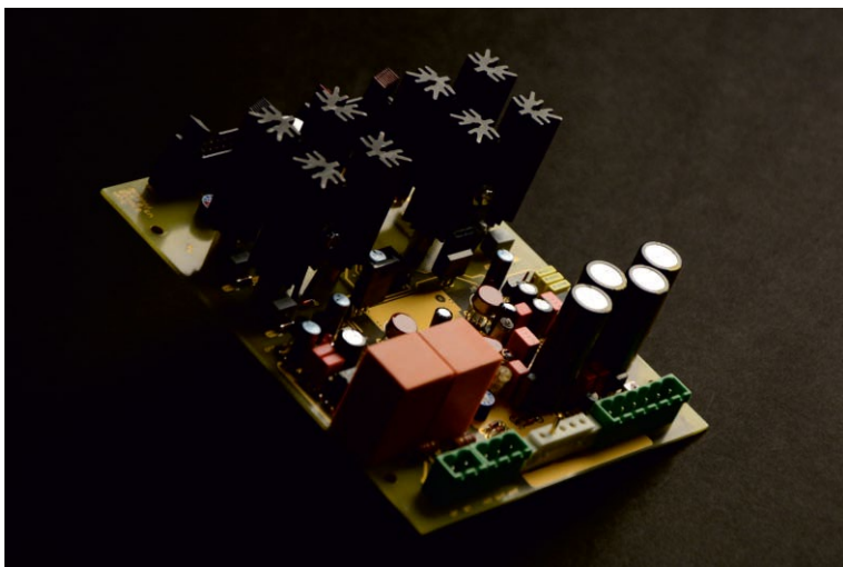
LDA driver board - HQS 9001 mono amplifier
