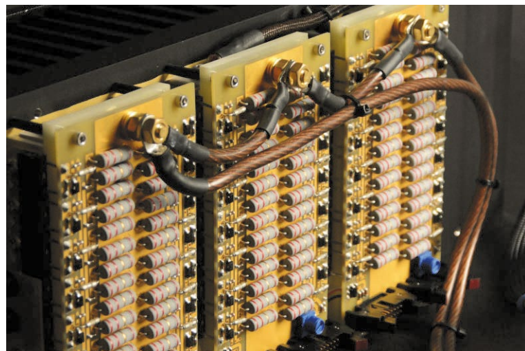
MTP output stage - HQS 9001 mono amplifier
